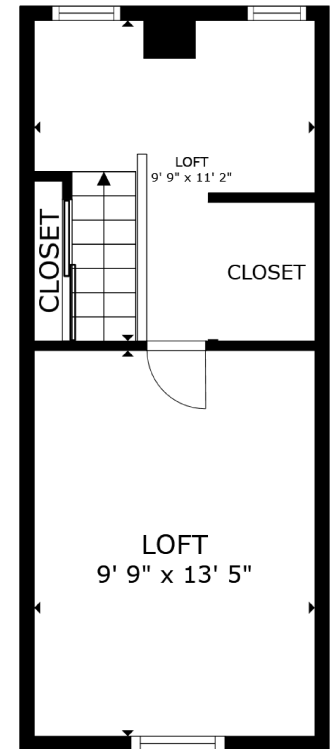
FLOOR 3
